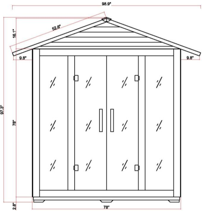
Front Panel Outside View
