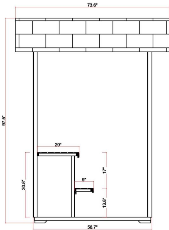
Side Panel Inside View
