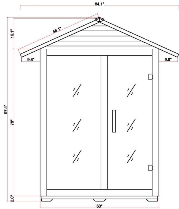
Front Panel Outside View
