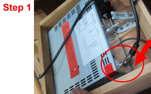
FIG-15 Screw CD Player into sauna room
